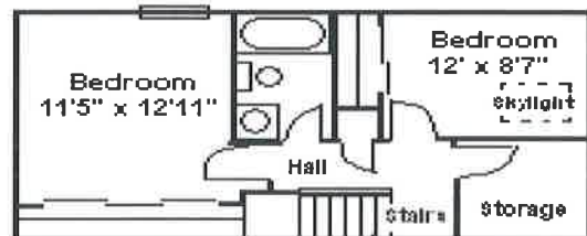
Second Floor
